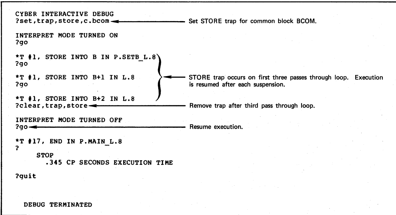
Figure 3-9. Debug Session Illustrating CLEAR,TRAP Command
