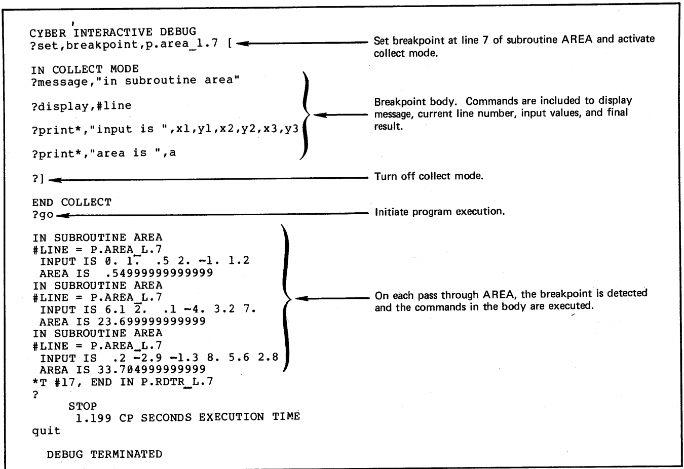
Figure 5-1. Debug Session Illustrating Breakpoint With Body
