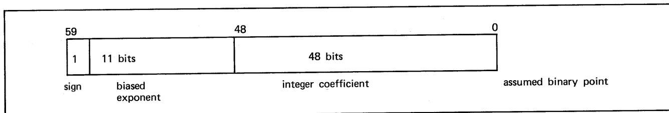
Figure C-1. Internal Floating Point Format
