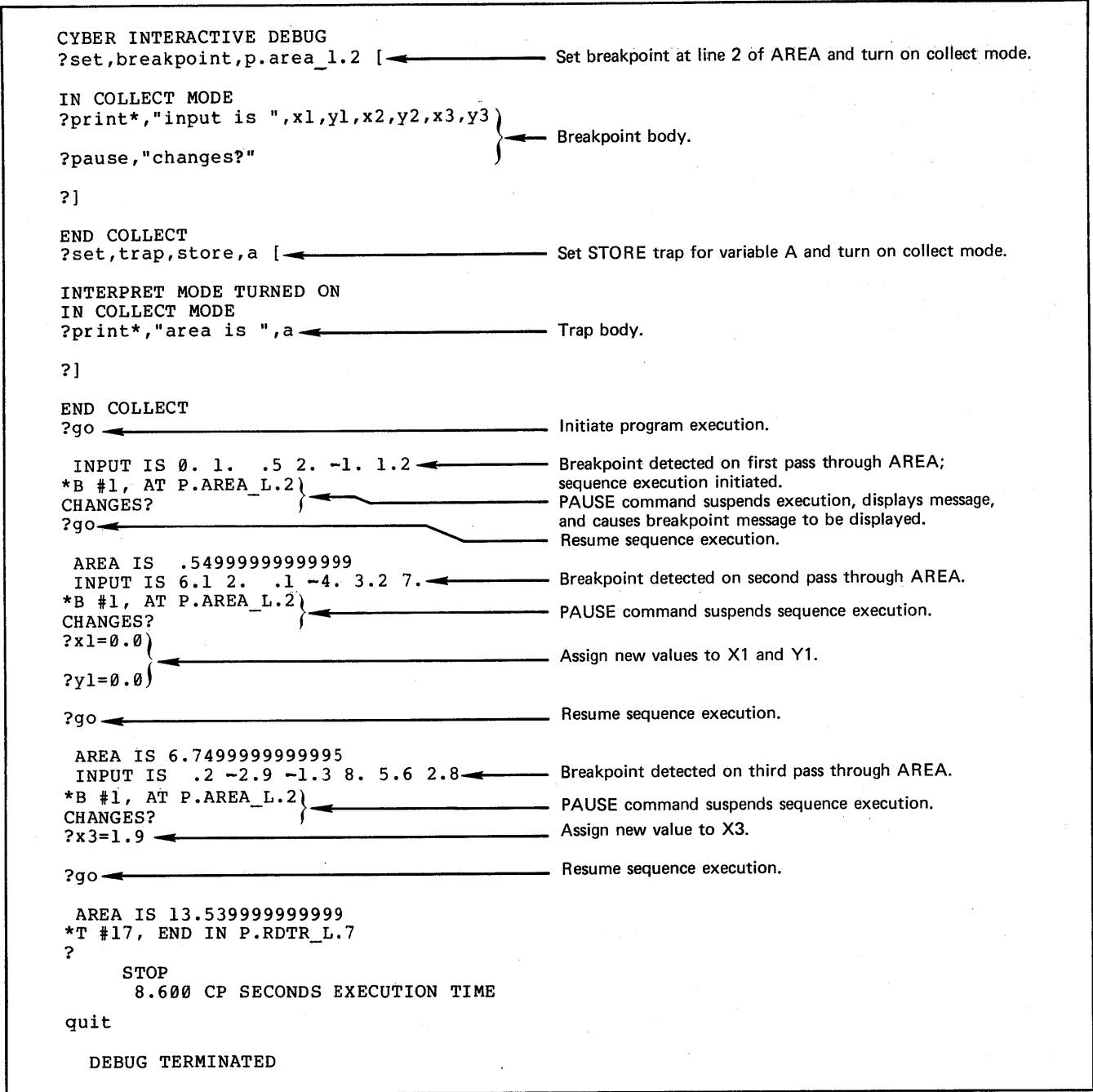
Figure 5-7. Debug Session Illustrating PAUSE Command
